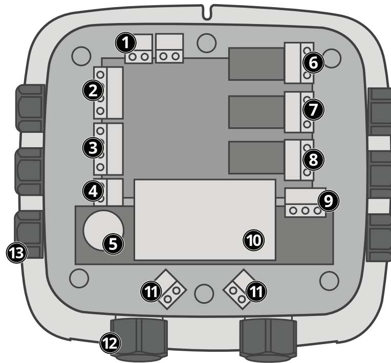
Figure 2-3 - MGS-402 Layout
