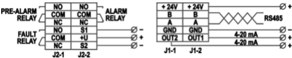
Electrical connections for version without 230 VAC PSU
