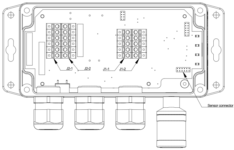
Detector version with 24 V DC power supply and without WiFi Module
